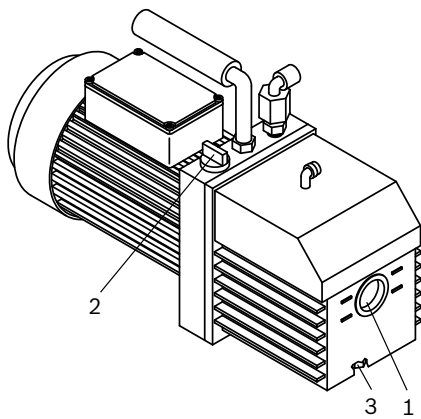
Fig. 22: Vacuum pump
